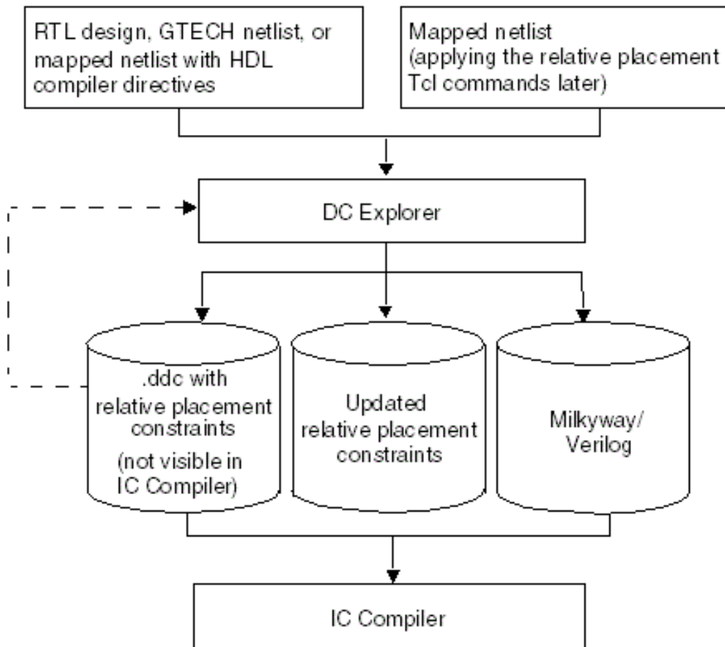
Figure 44 Overview of the Relative Placement Flow
