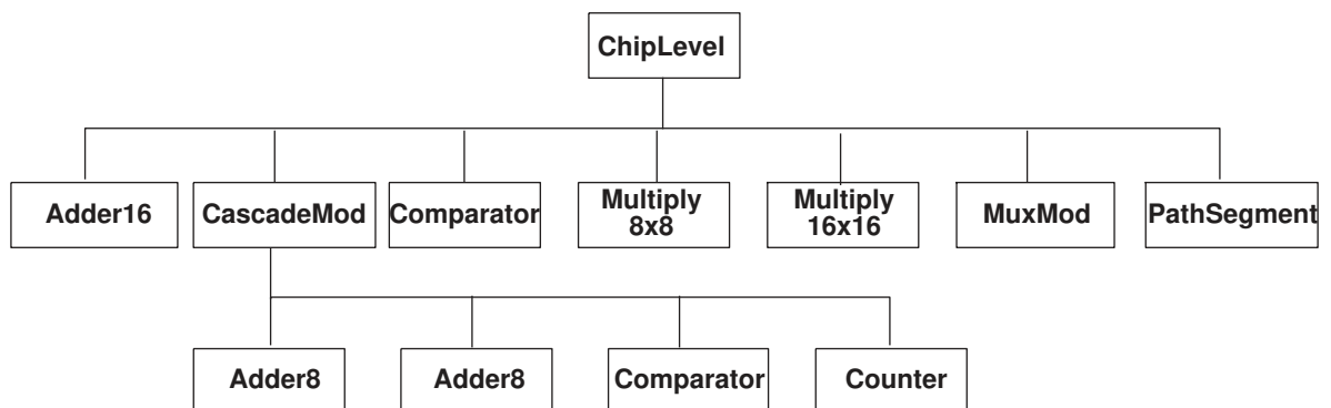
Figure 93 Hierarchy for the Design Example
