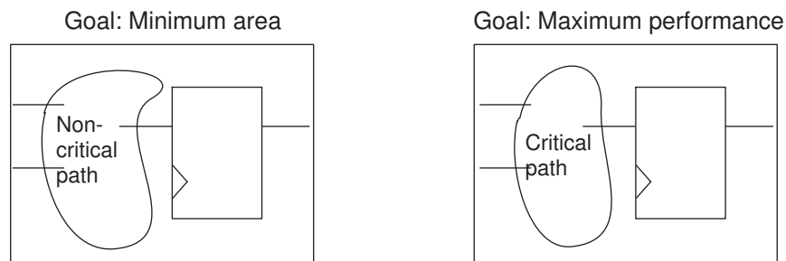
Figure 87 Blocks With Different Constraints
