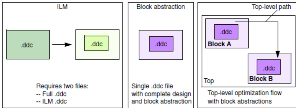
Figure 67 ILM and Block Abstraction Comparison
