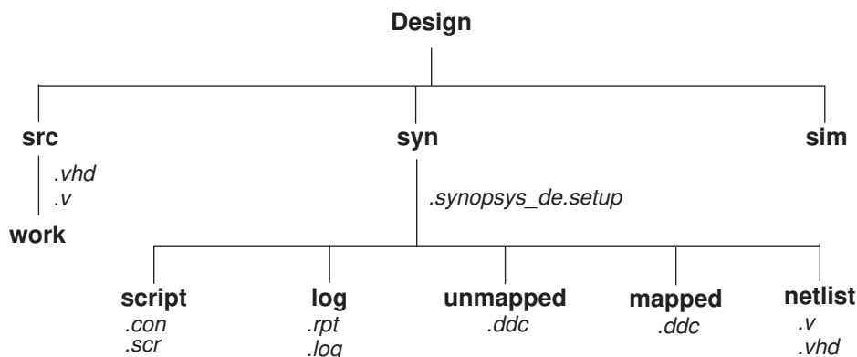
Figure 82 Top-Down Compile Directory Structure
