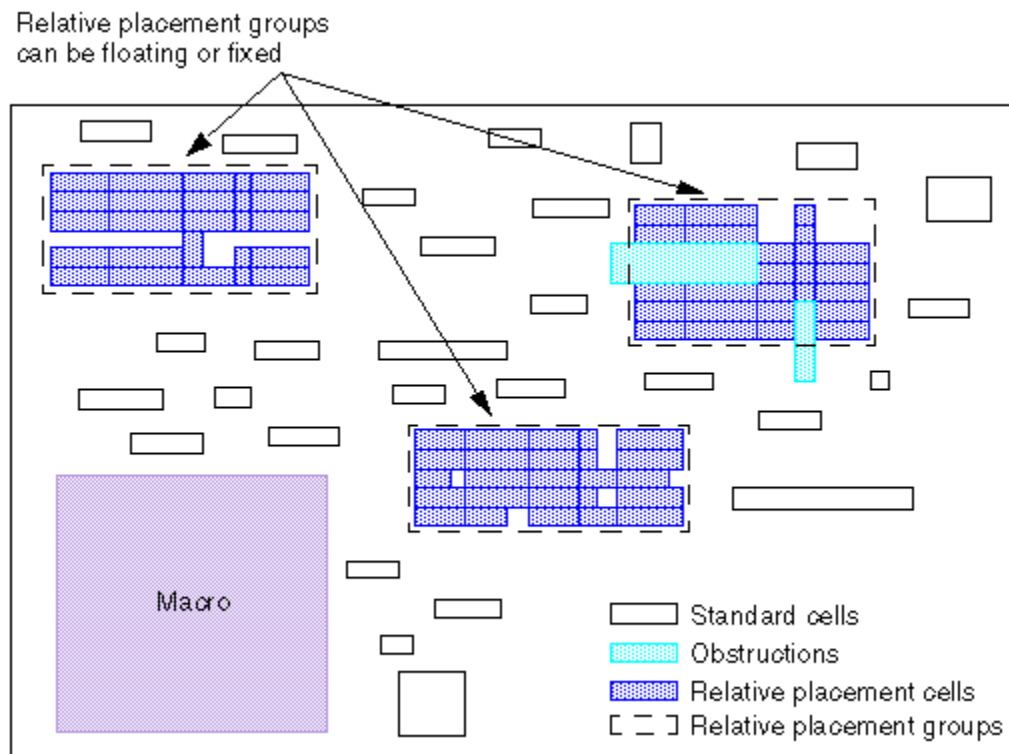
Figure 43 Relative Placement in a Floorplan
