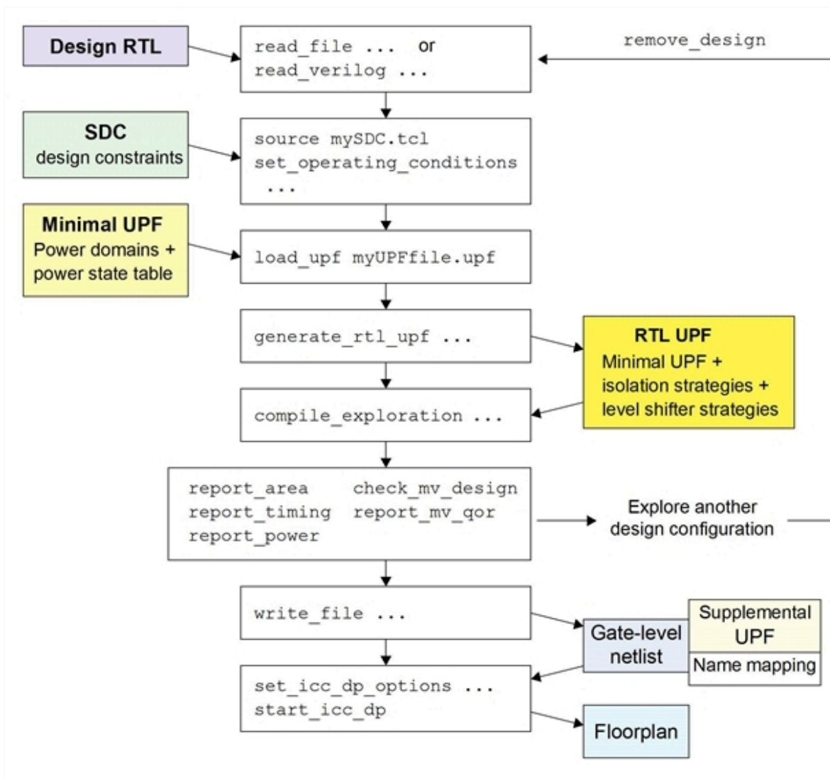
Figure 34 Design Exploration Flow With UPF
