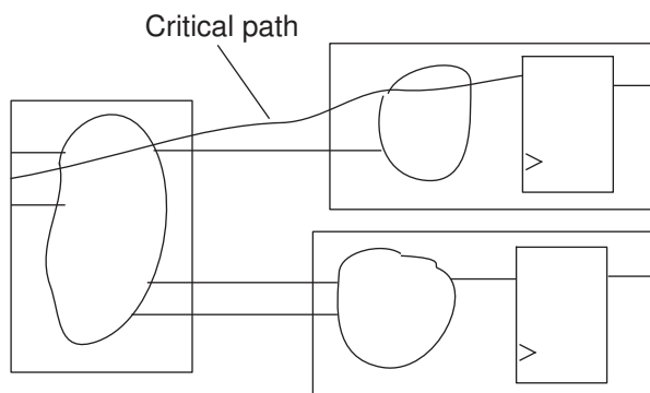
Figure 84 Poor Partitioning of Related Logic
