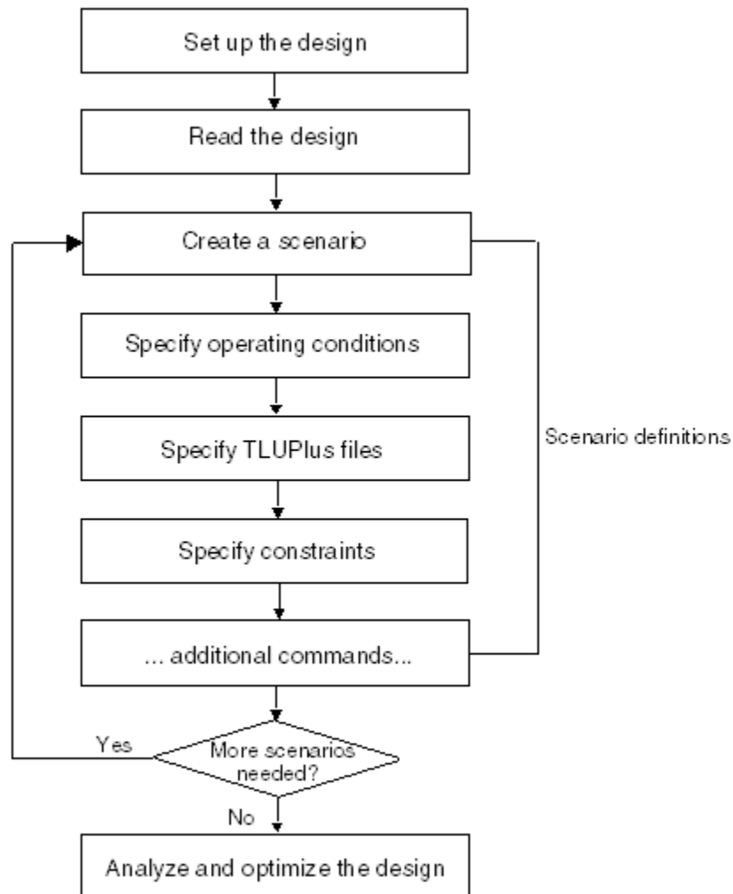
Figure 58 Basic Multicorner-Multimode Flow
