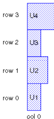
Figure 47 Bottom-Left Aligned Relative Placement Group
