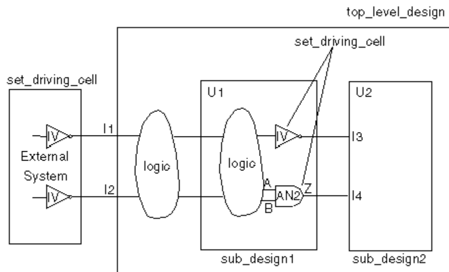
Figure 24 Drive Characteristics
