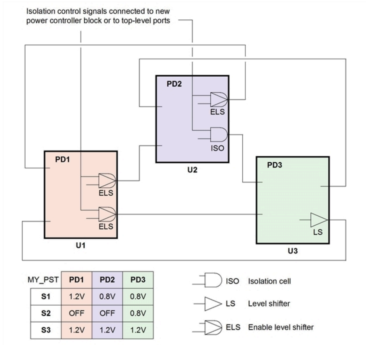
Figure 35 Isolation and Level Shifter Cells Inserted by DC Explorer
