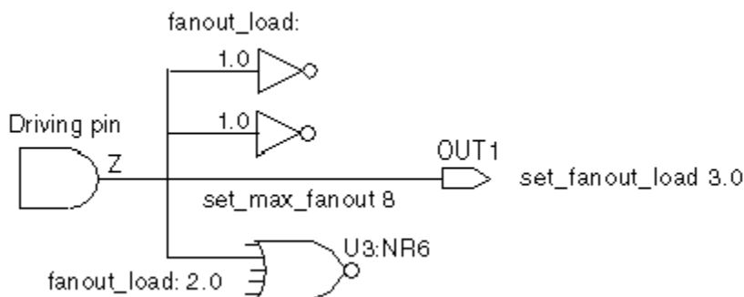
Figure 29 Calculation of Maximum Fanout
