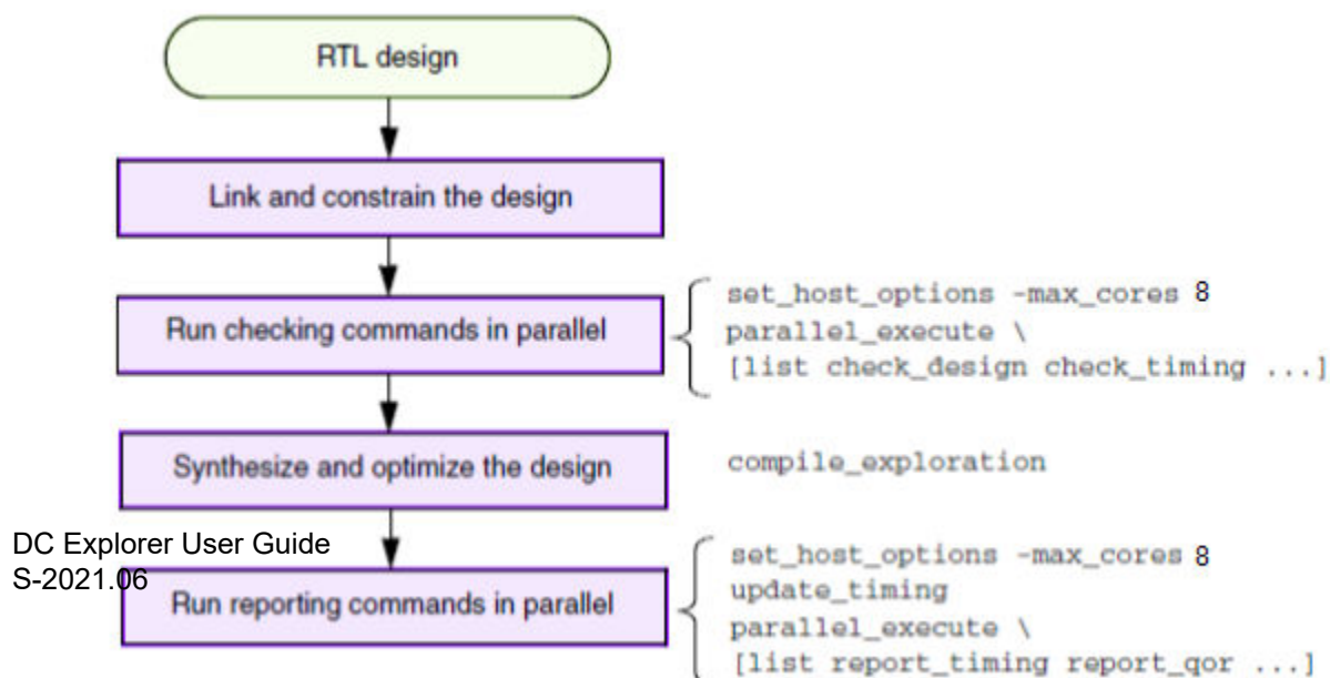
Figure 2 Parallel Command Execution in the DC Explorer Design Flow
