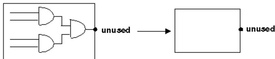
Figure 26 Minimizing Logic Driving an Unconnected Output Port
