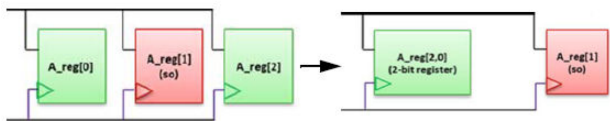
Figure 64 Noncontiguous Multibit Mapping
