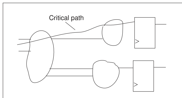
Figure 85 Keeping Related Logic in the Same Block
