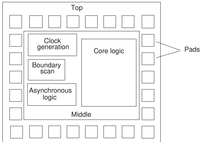
Figure 90 Recommended Top-Level Partitioning
