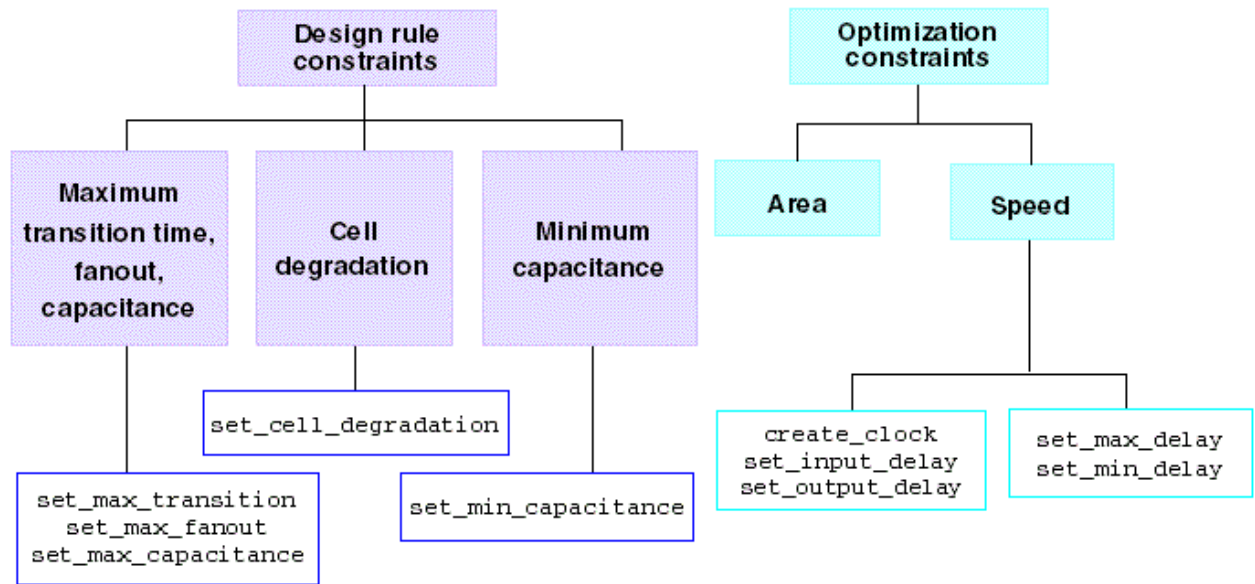
Figure 27 Major DC Explorer Constraints
