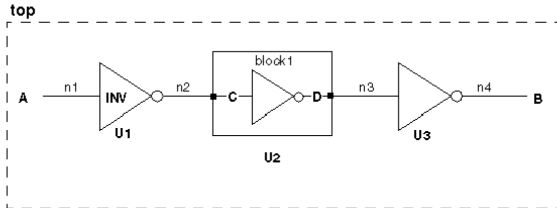
Figure 30 Characterizing Drive, Timing, and Load Values of a Combinational Design
