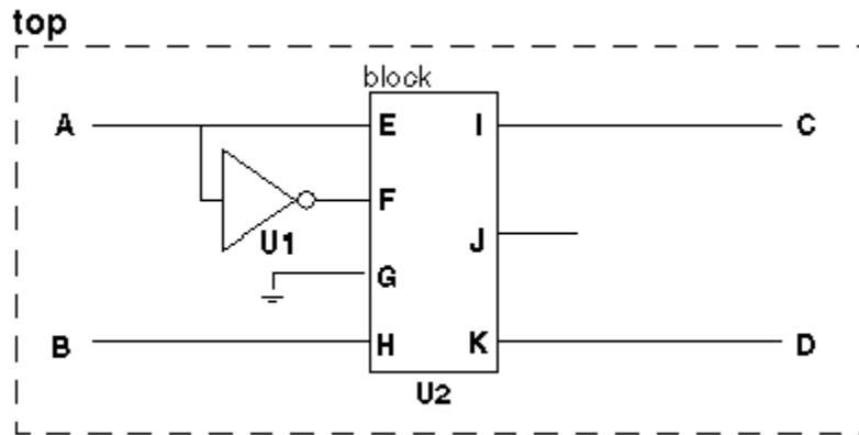
Figure 32 Characterizing Port Connection Attributes
