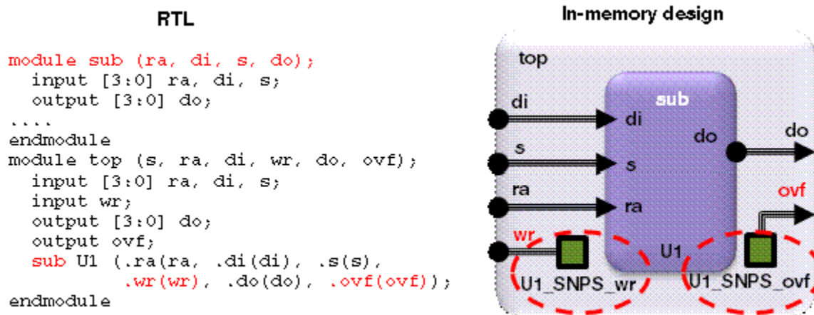
Figure 7 Example of Missing Pins in Logic Libraries
