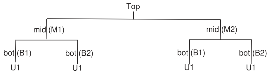
Figure 22 Cell Instances U1 in the bot Design
