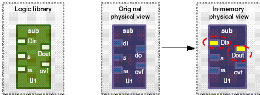
Figure 13 Example of Pin Mapping Between Logic Library and Physical Library
