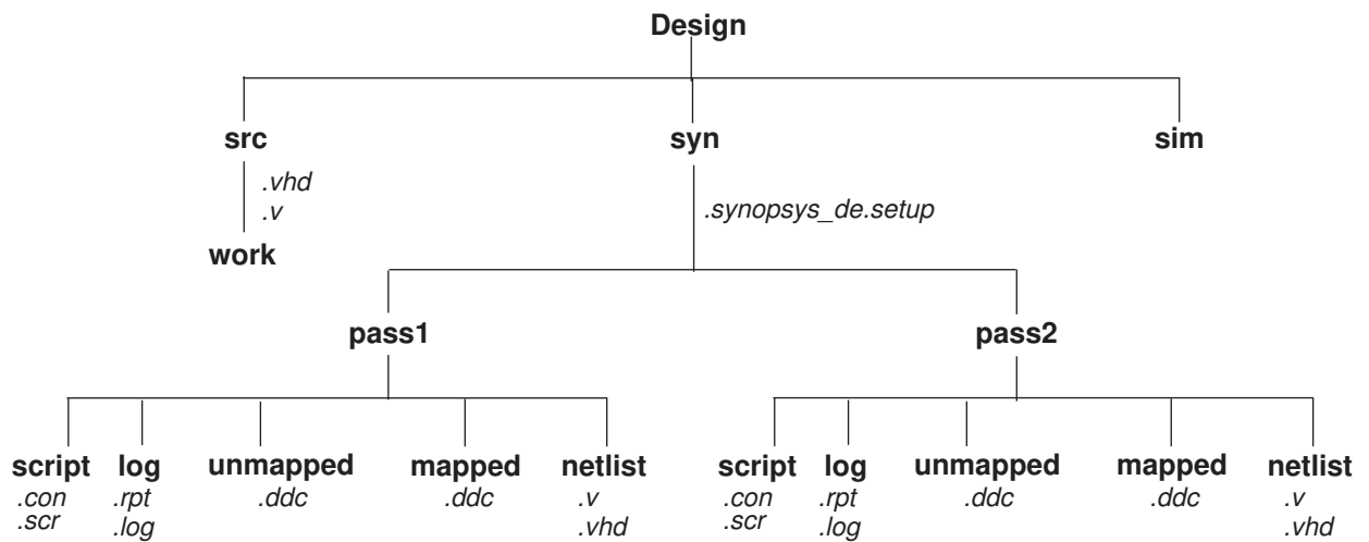
Figure 83 Bottom-Up Compile Directory Structure
