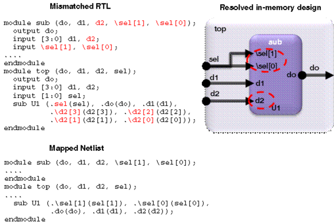
Figure 11 Example of Bus and Bus-Blasted Naming Styles
