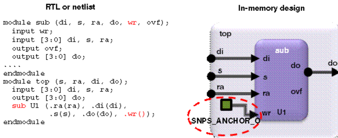
Figure 14 Example of Unconnected Interface Pins
