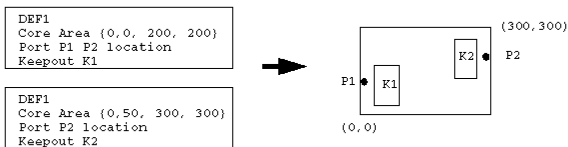
Figure 37 Incremental Extraction With the extract_physical_constraints Command
