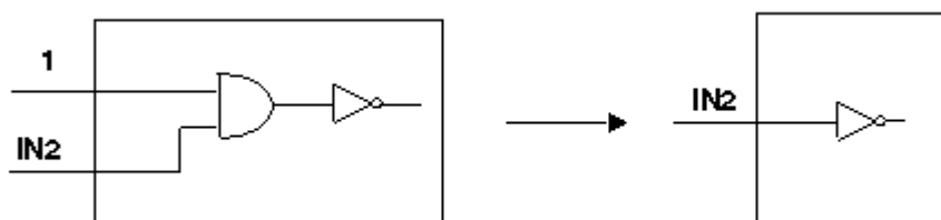
Figure 25 Simplified Input Port Logic
