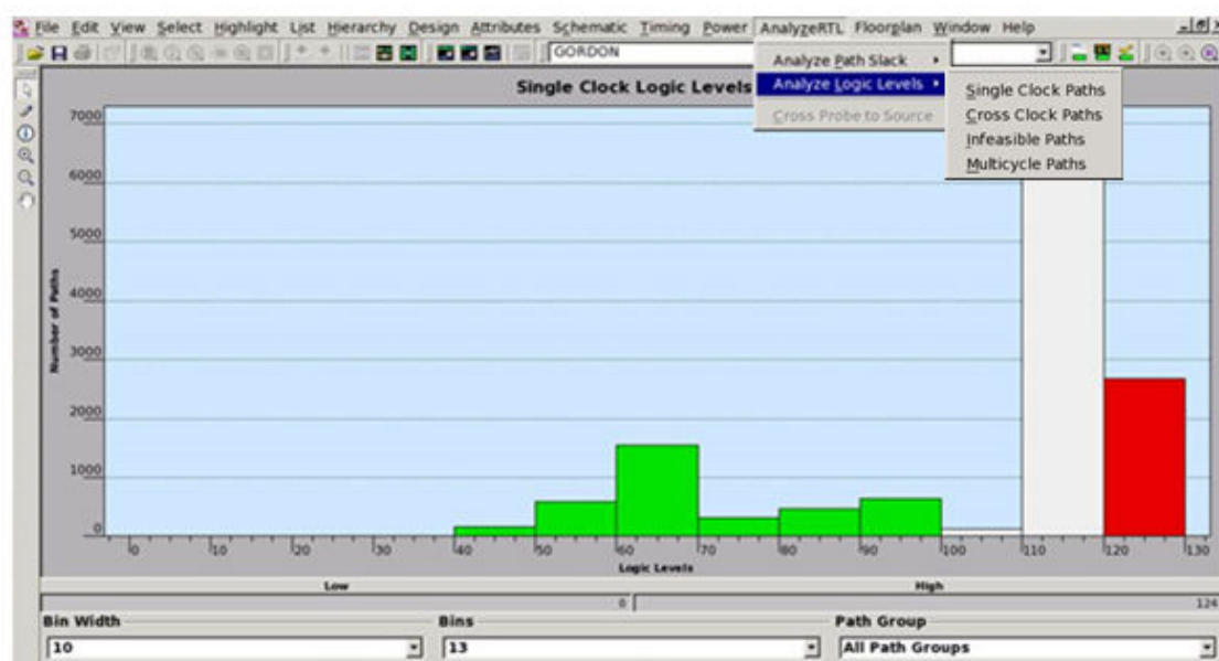
Figure 77 Logic-Level Histogram
