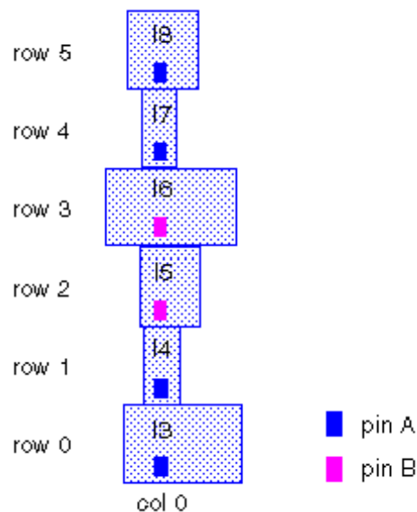
Figure 50 Relative Placement Group Aligned by Pins
