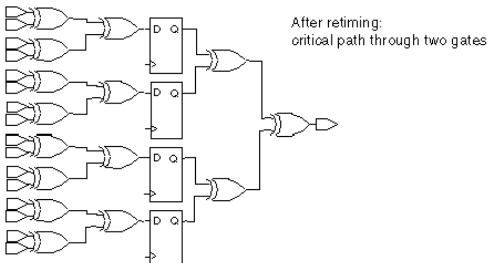
Figure 60 Circuit After Retiming
