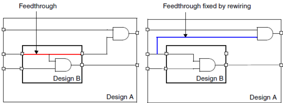
Figure 62 Feedthrough Fixed by Rewiring Across the Hierarchy
