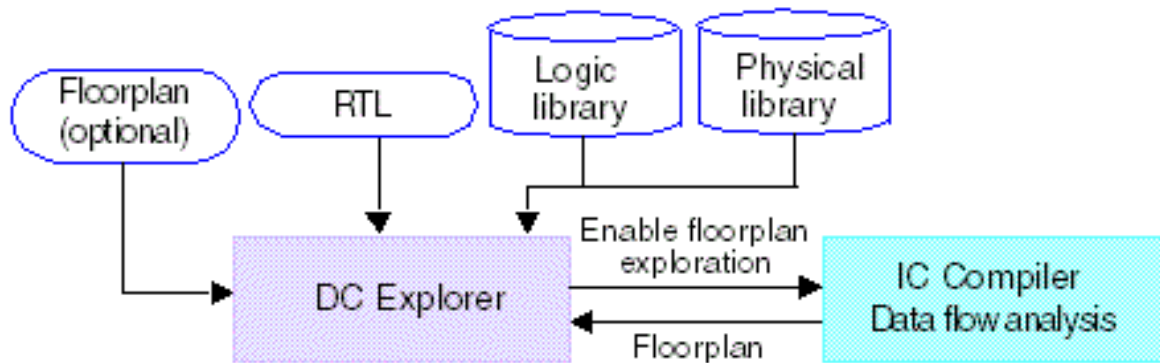
Figure 70 Early Floorplanning Using Data Flow Analysis
