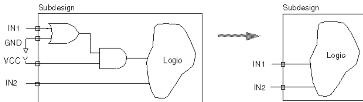
Figure 53 Benefits of Boundary Optimization
