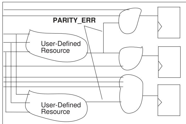
Figure 89 Duplicating User-Defined Resources
