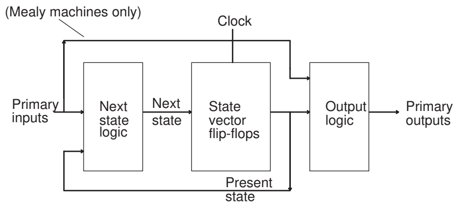
Figure 91 Finite State Machine Architecture
