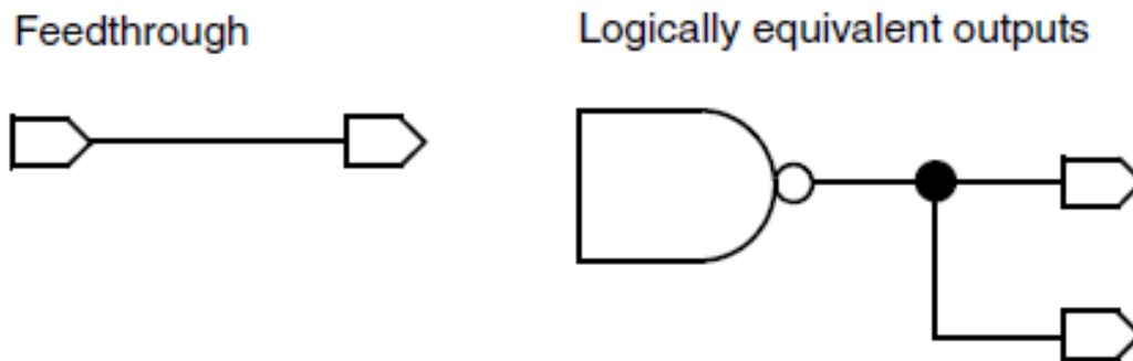
Figure 61 Nets Connected to Multiple Ports
