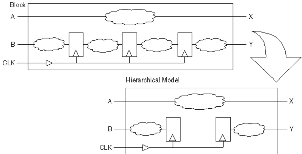
Figure 65 A Block and Its Hierarchical Model
