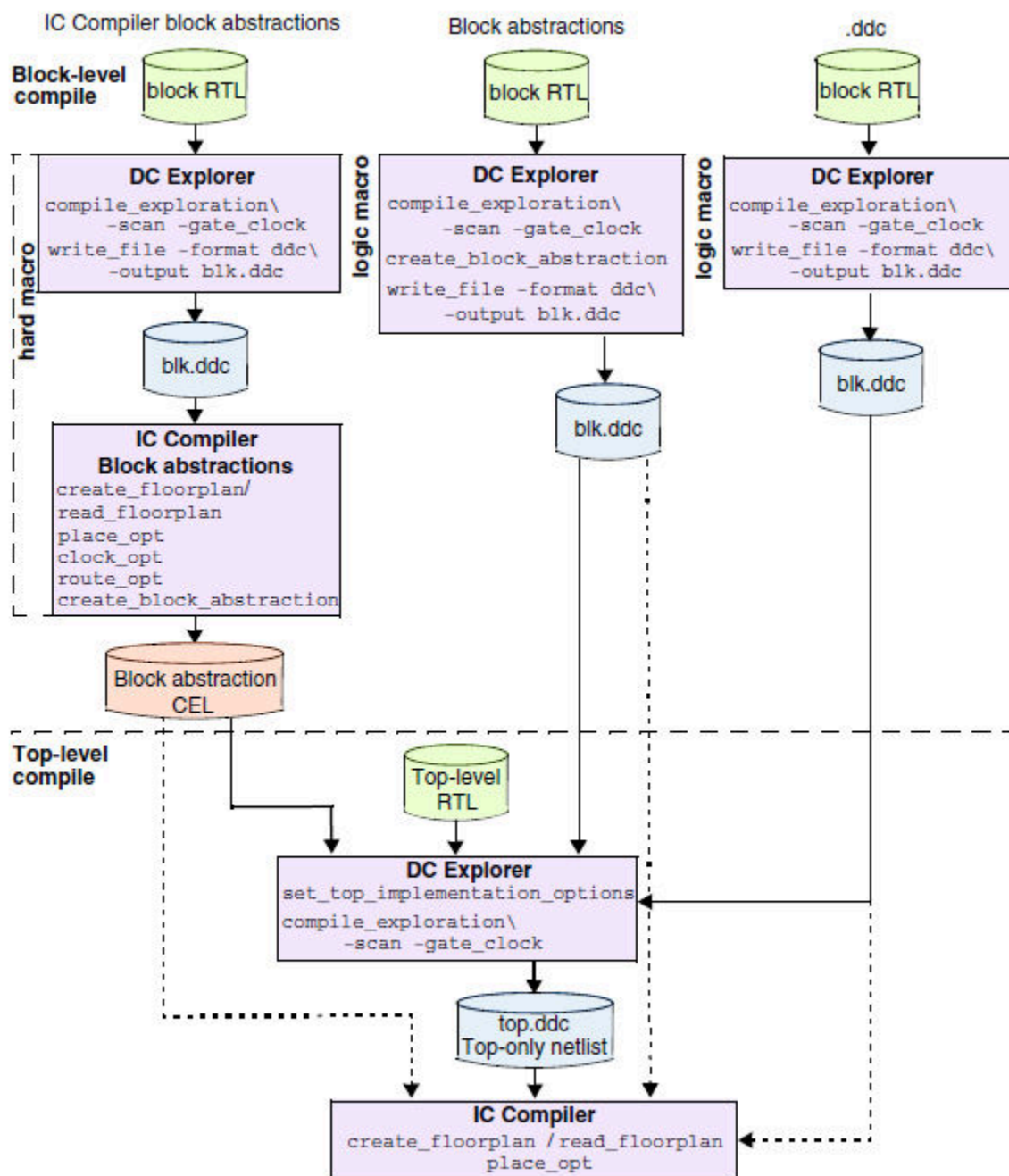
Figure 52 Overview of the Hierarchical Flow for Designs Containing Block Abstractions
