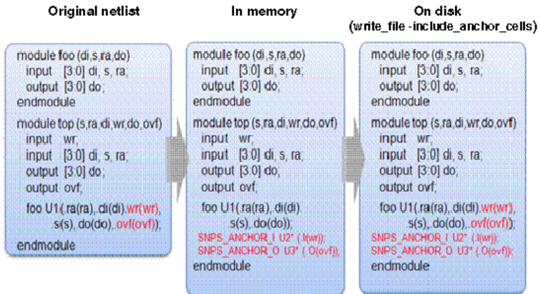
Figure 15 anchor Cells Support in Netlist
