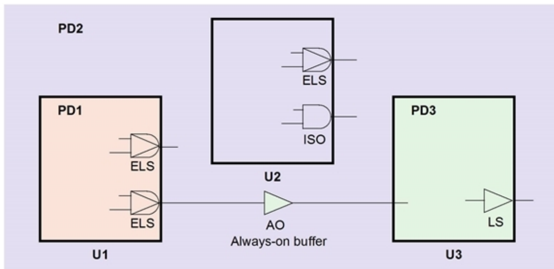
Figure 36 Always-On Buffer Inserted by the DC Explorer Tool
