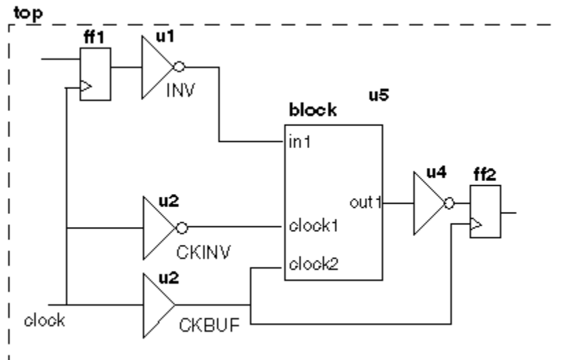
Figure 31 Characterizing Sequential Design Drive, Timing, and Load Values
