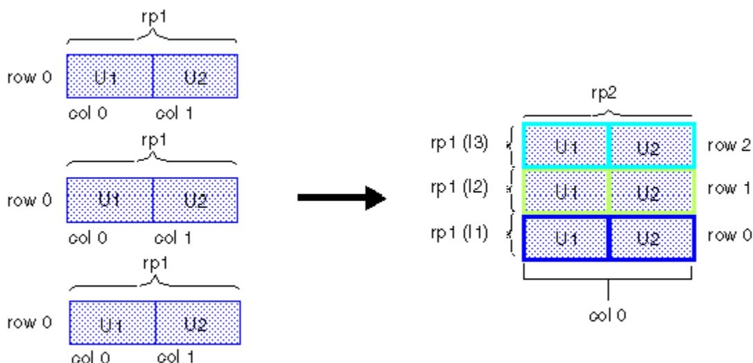
Figure 46 Instantiating Groups in a Hierarchical Group
