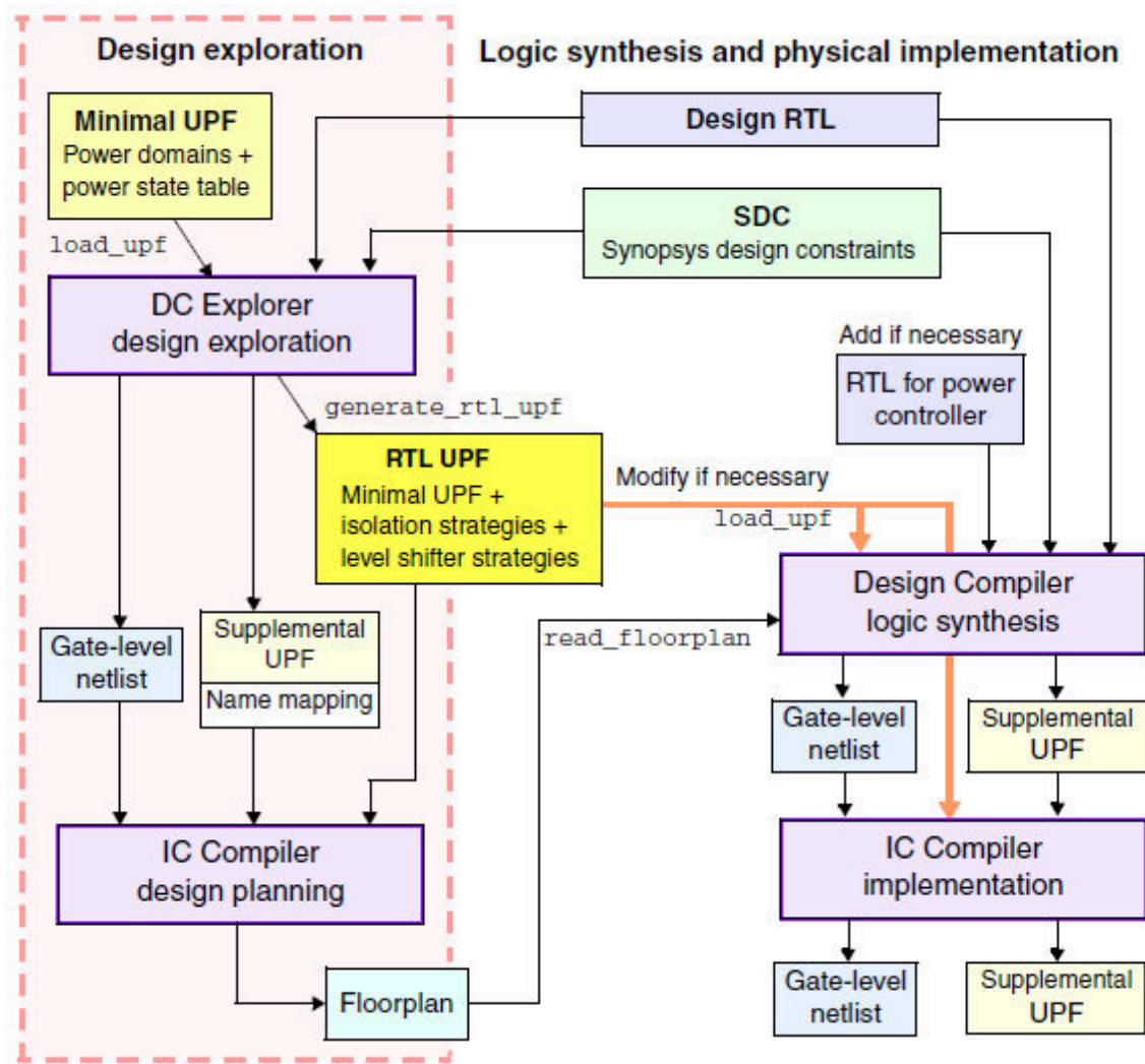
Figure 33 Design Exploration, Synthesis, and Implementation Flow With UPF
