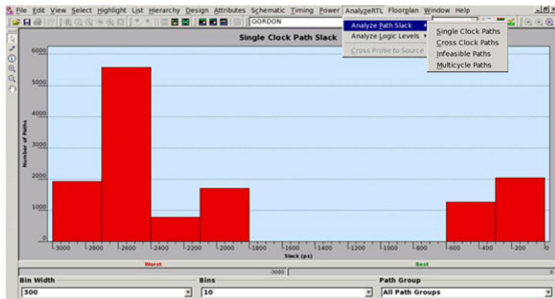
Figure 76 Path Slack Histogram
