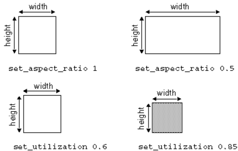
Figure 38 Using the set_aspect_ratio and set_utilization Commands
