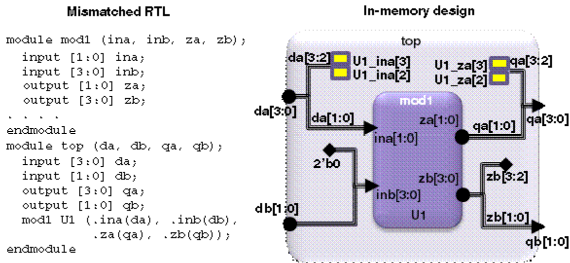
Figure 10 Example of Port Width Mismatches
