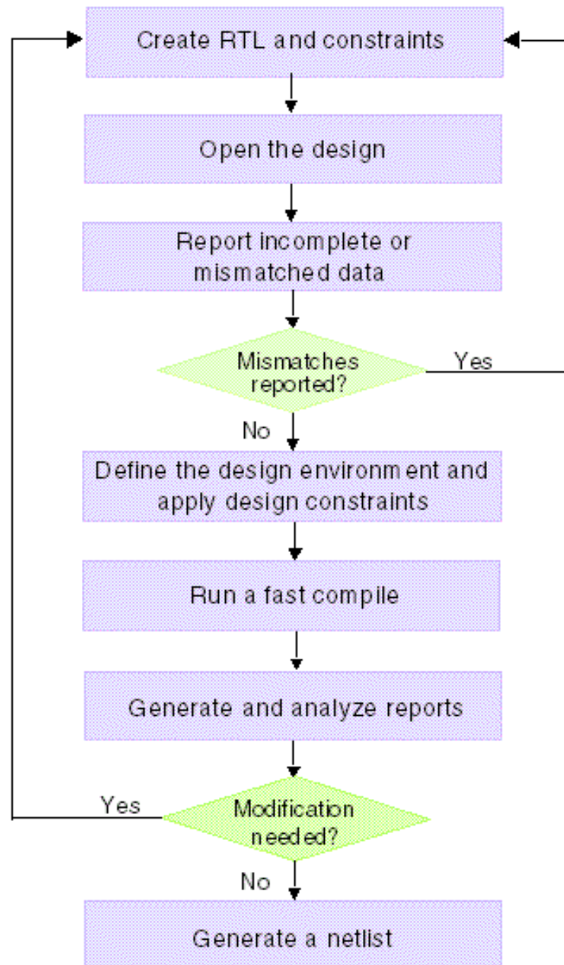
Figure 1 Design Flow in DC Explorer
