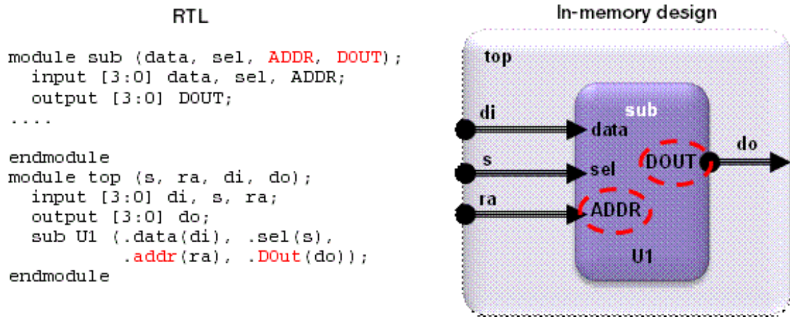
Figure 4 Example of Case Mismatches Between Pin Name
