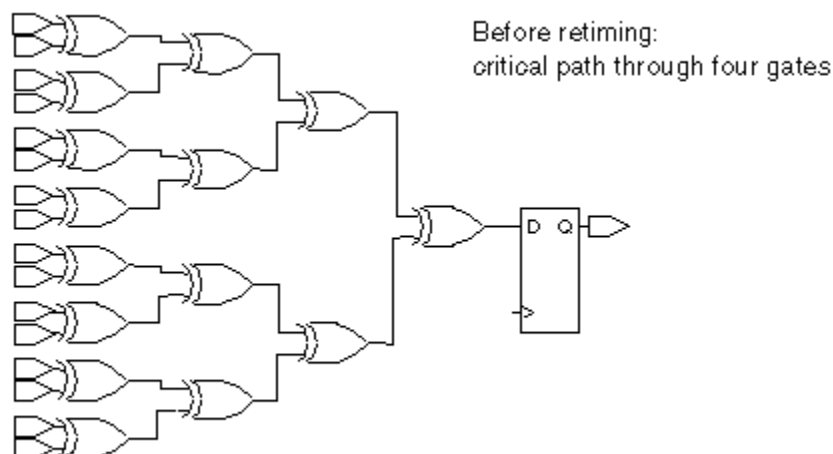
Figure 59 Circuit Before Retiming
