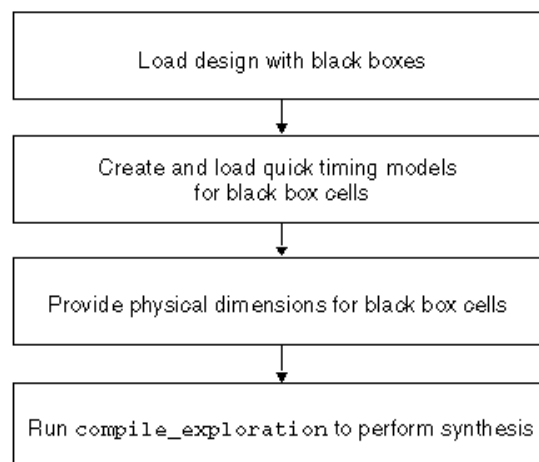
Figure 3 Supported Black Box Flow
