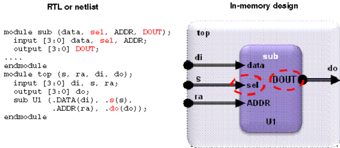
Figure 12 Pin Mapping Between Top-Level Instantiations and RTL Blocks
