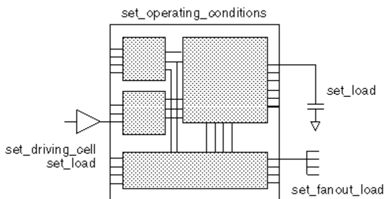
Figure 23 Commands Used to Define the Design Environment
